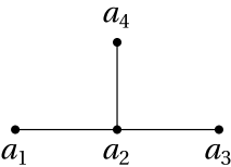
FIGURE 1. Tree G^T .
