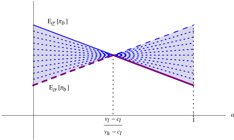
FIGURE 1. Expected payoffs E_\sigma[\pi_b] for \sigma \in [\underline{\sigma}, \overline{\sigma}] .
