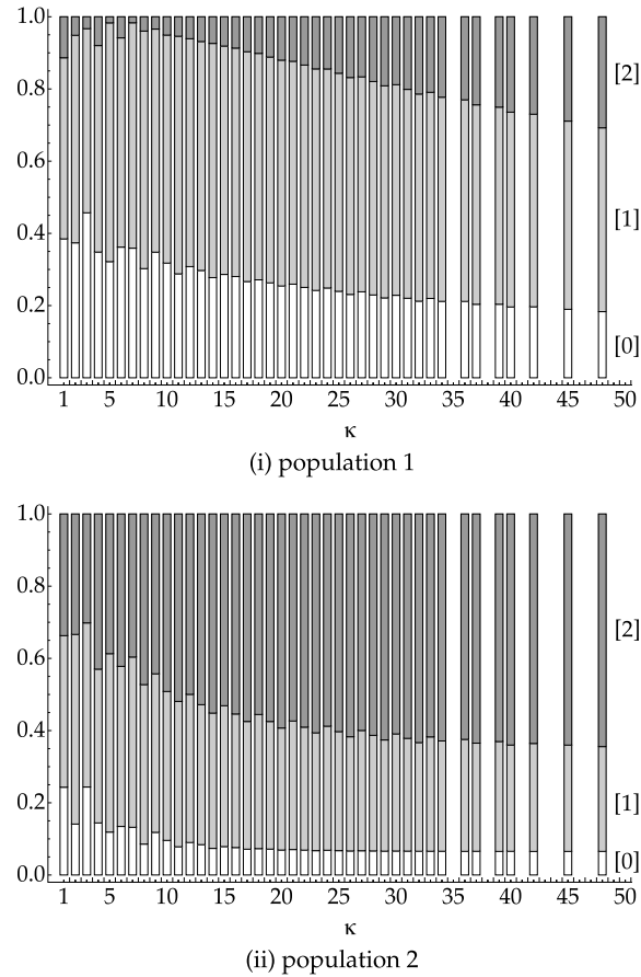
FIGURE 3. The stable interior rest point of the \text{BEP}(\tau^{\text{all}}, \kappa, \beta^{\text{min}}) dynamic in the centipede game of length d = 4 , \kappa = 1, \dots, 50 . Stacked bars, from the bottom to the top, represent weights on strategies [0], [1], and [2].
