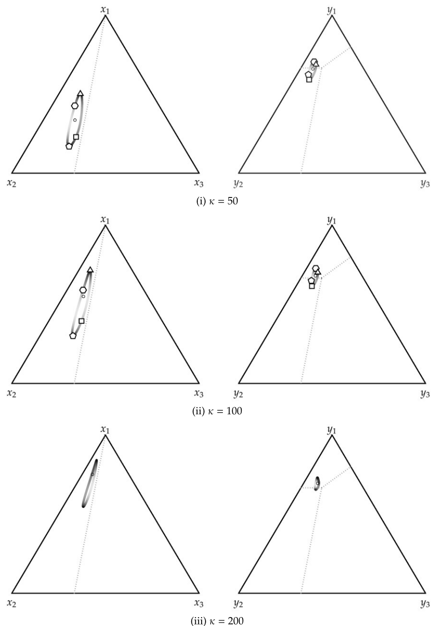
FIGURE 5. Stable cycles in centipede of length d = 4 under \text{BEP}(\tau^{\text{all}}, \kappa, \beta^{\min}) dynamics for \kappa = 50, 100 , and 200 . Lighter shading represents faster motion. The small circles represent the unstable interior rest points. For \kappa = 50 and 100 , shapes synchronize positions along the cycle.
