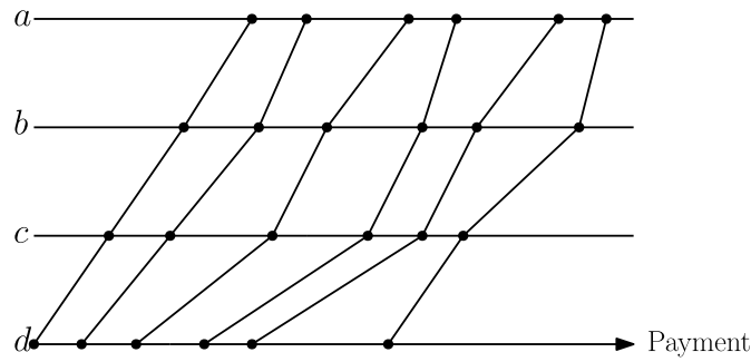
FIGURE 2. A preference and its indifference diagram for the case a > b > c > d .
