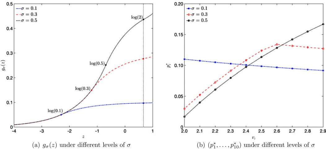
FIGURE 1. The functions g_\sigma(z) and (p_1^*, \dots, p_{10}^*) under different levels of \sigma .
