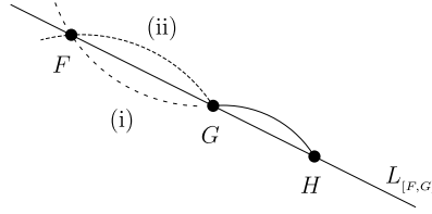
FIGURE 4. G = \alpha_0 F + (1 - \alpha_0)H , \alpha_0 \leq \frac{1}{2} .
