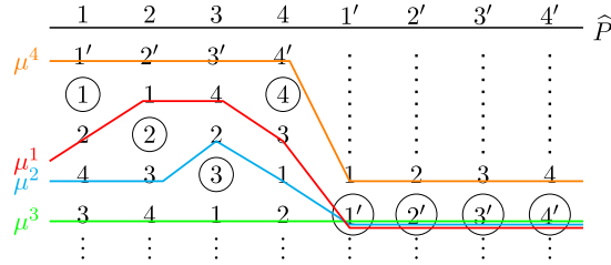
FIGURE 15. Problem \hat{P} .
