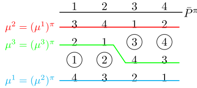
FIGURE 19. Permutated problem \bar{P}^\pi after permuting problem \bar{P} of Figure 18 with \pi = (1324) .
