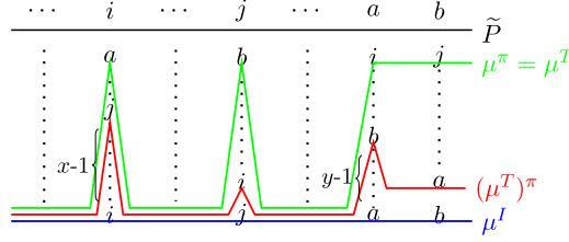
FIGURE 11. Problem \tilde{P} , after swapping the positions of \mu^\pi and (\mu^T)^\pi in problem \hat{P}^\pi in Figure 10.
