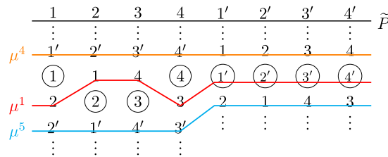
FIGURE 16. Problem \tilde{P} .
