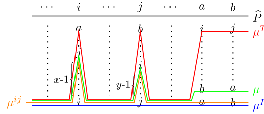
FIGURE 9. Problem \hat{P} = (\hat{N}, \hat{R}) .
