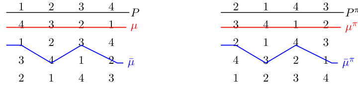
FIGURE 28. An example of violation of anonymity condition by \delta^A .
