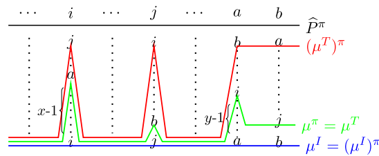
FIGURE 10. Problem \hat{P}^\pi after permuting problem \hat{P} in Figure 9 with \pi = (aj) .
