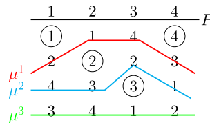
FIGURE 2. In the problem above, an example for an interval is [\mu^1, \mu^3]_{R_1} = \{2, 4, 3\} and the length of this interval is |\mu^1, \mu^3|_{R_1} = 2 . The matching \mu^2 is between \mu^1 and \mu^3 while the identity matching is denoted with circles.
