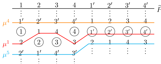
FIGURE 16. Problem \tilde{P} .
