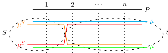
FIGURE 3. The general view of the decomposition lemma.
