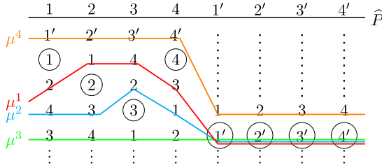
FIGURE 15. Problem \hat{P} .
