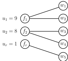
FIGURE 3. Matching m^* : The unique stable matching.
