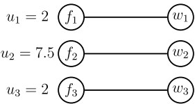
FIGURE 6. Matching m^* : Unique stable matching.
