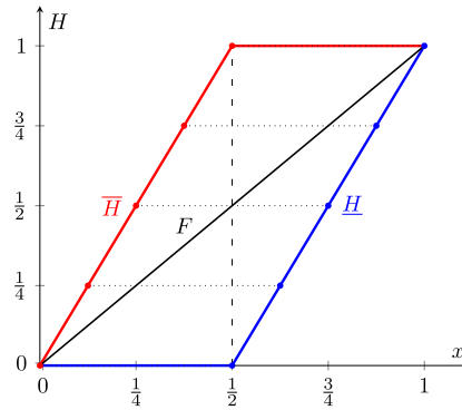
FIGURE 1. Implementable distributions of posterior medians. When the prior F is uniform on [0, 1] , \overline{H} and \underline{H} are the lowest and highest implementable distributions of posterior medians. A distribution H is implementable if and only if \underline{H} \leq H \leq \overline{H} . Optimizing a linear functional over distributions of posterior medians requires taking the optimal selection from each horizontal dotted line. For example, the blue (red) dots are the optimal selections for an increasing (decreasing) objective function.
