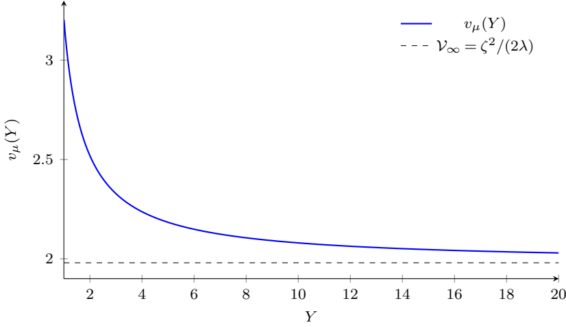
FIGURE 2. Solution of equation (5.17) for \mu = 1 and Y \geq 1 . Parameters are \zeta = 2 , \Delta = 1 , and r = 0.01 (so \lambda = r + \Delta ). The solid line plots v_\mu(Y) , while the dashed line represents the asymptotic value \mathcal{V}_\infty = \zeta^2/(2\lambda) .
