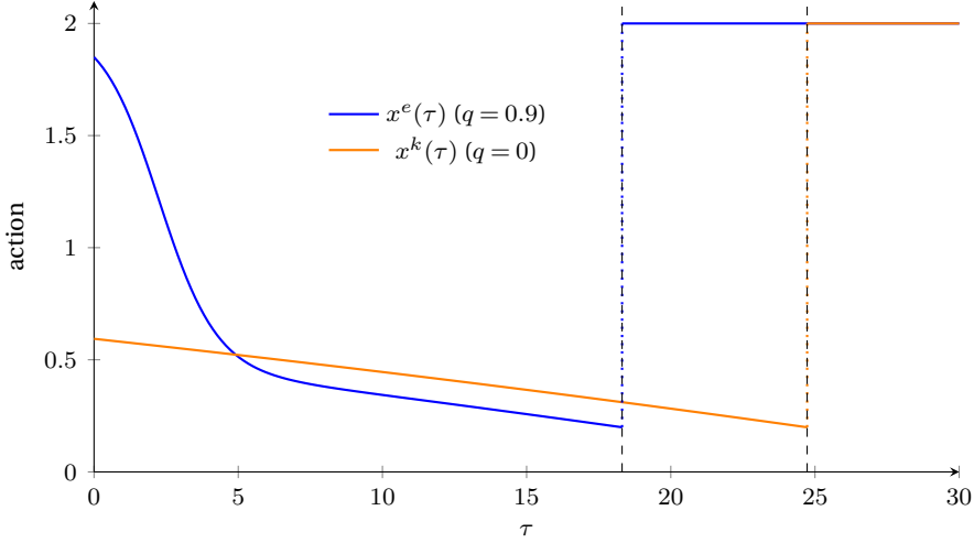
FIGURE 1. Optimal actions x^e(\tau) ( q = 0.9 ) and x^k(\tau) ( q = 0 ) for \bar{X} = 10 . Parameters are \zeta = 2 , r = 0.01 , \Delta = 1 , \lambda = r + \Delta = 1.01 . Vertical dashed lines indicate dates \bar{T}^e and \bar{T}^k .
